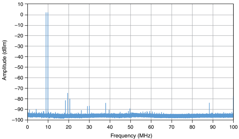
Figure 10. 9.5 MHz and 10.5 MHz Dual-Tone Spectrum 23 , Measured
