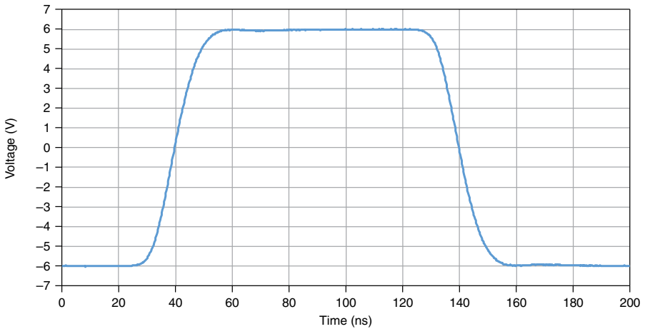
Figure 7. Square Waveform Step Response at 12 V_{pk-pk} , Measured
