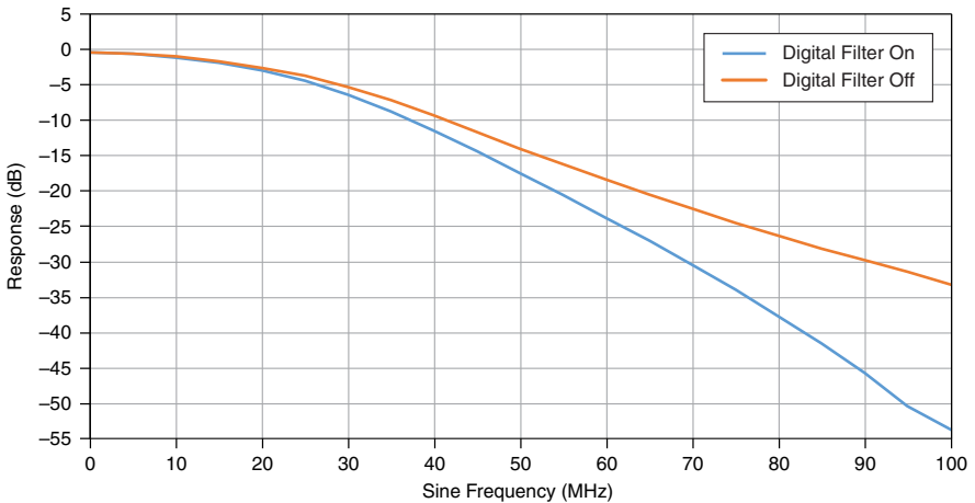
Figure 8. Magnitude Response 21 , Measured
