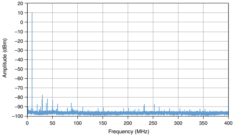
Figure 3. 10 MHz Spectrum 13 at 2 V pk-pk , Measured
