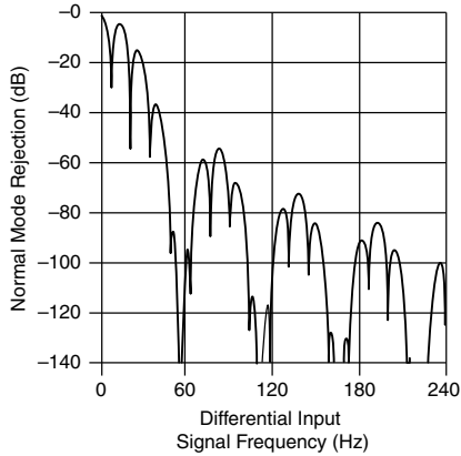
Figure 2. High-Resolution Filter Response 4, 5
