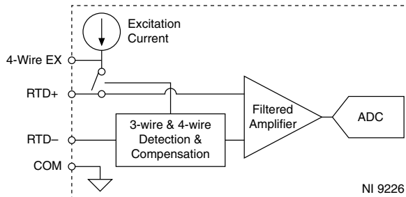
Figure 1. Input Circuitry for One Channel of the NI 9226
