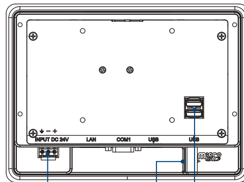
Power Input
