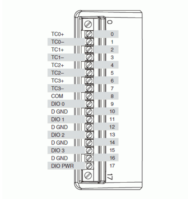
NI WSN-3212 Pinout
