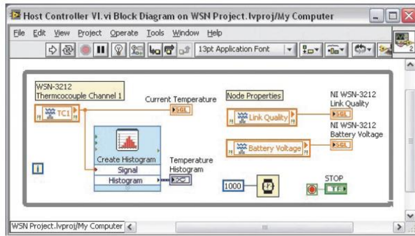
Figure 2. Extracting NI WSN Measurement Data Using LabVIEW and I/O Variables
