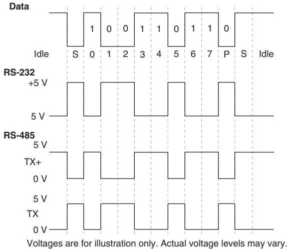
Figure 12. UART Data Frame Example
