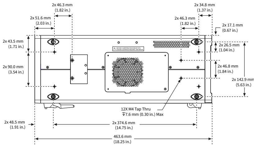
Figure 1. PXle-1092 Chassis Dimensions (Bottom)
