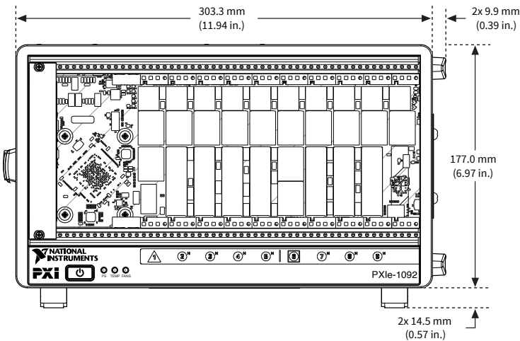
Figure 1. PXIe-1092 Chassis Dimensions (Front)
