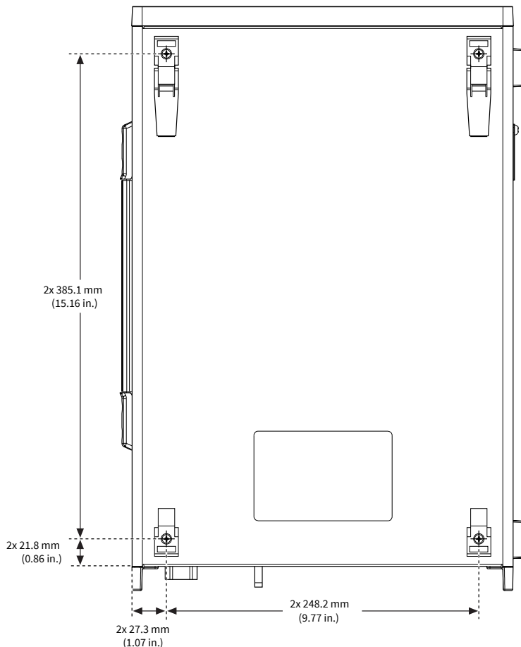
Figure 1. PXle-1092 Chassis Dimensions (Bottom)
