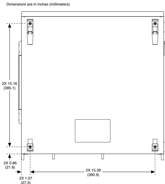
Figure 2. PXle-1095 Chassis Dimensions (Bottom)
