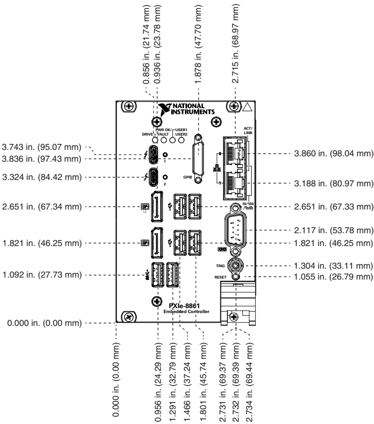
Figure 1. PXIe-8861 Front Panel Layout and Dimensions
