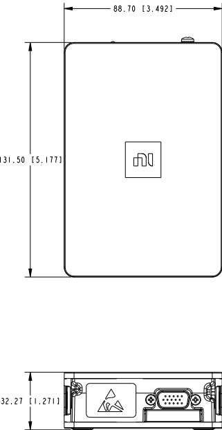
Figure 3. cDAQ-9170 Dimensions
