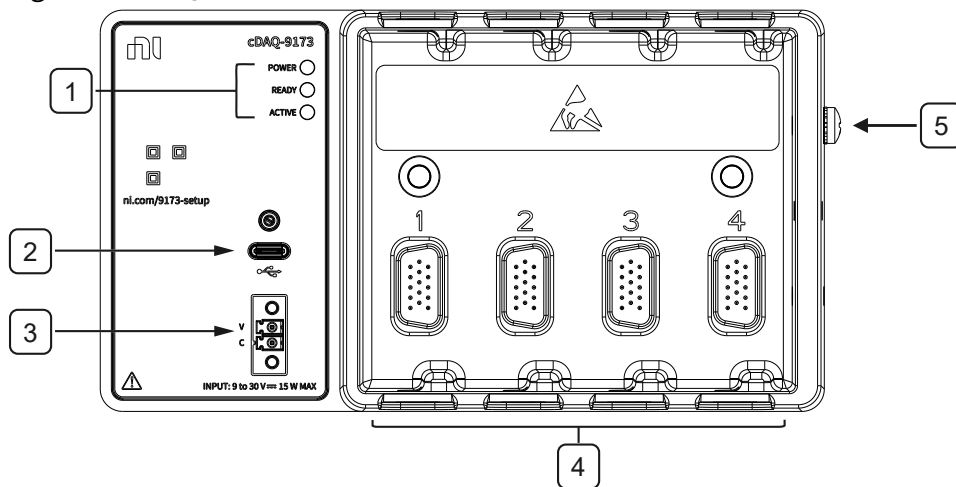
Figure 2. cDAQ-9173 Front Panel
