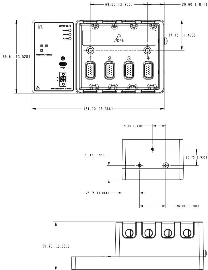
Figure 3. cDAQ-9173 Dimensions
