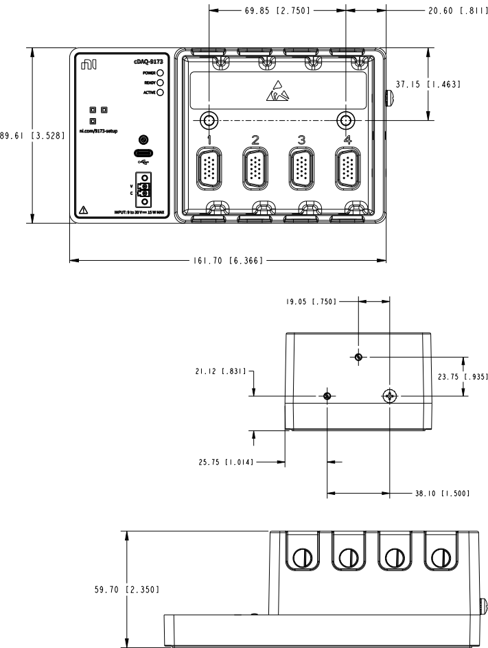
Figure 3. cDAQ-9173 Dimensions
