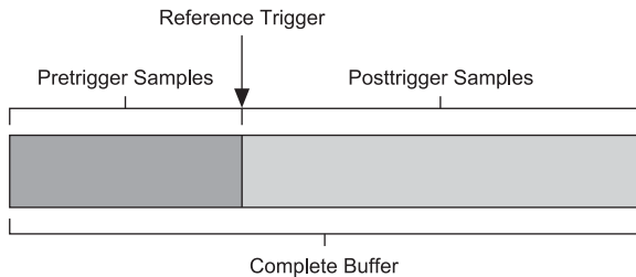
Figure 36. Reference Trigger Final Buffer
