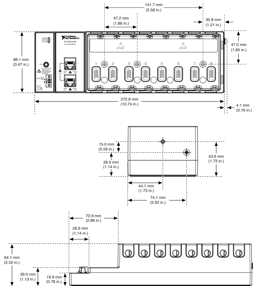
Figure 1. cDAQ-9189 Dimensions
