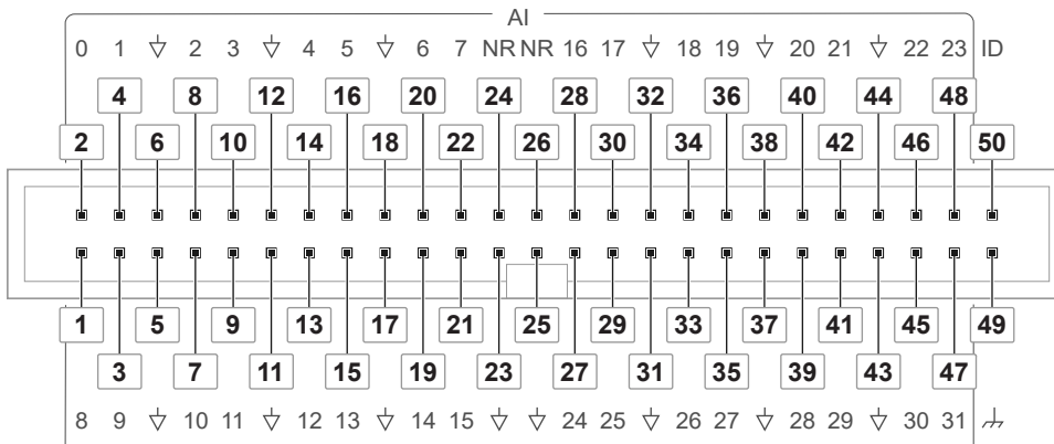
Figure 3. USB-6453 (OEM) AI Connector Pinout
