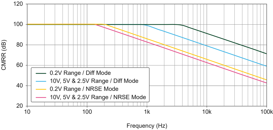
Figure 8. USB-6453 (Revision F and subsequent revisions) and USB-6453 (OEM) CMRR versus
