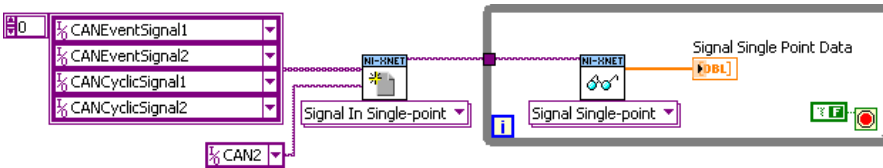
Figure 4. NI-XNET Code Without Sessions
