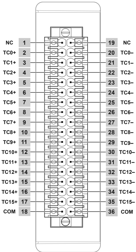
Figure 1. NI-9313 Connector Pinout
