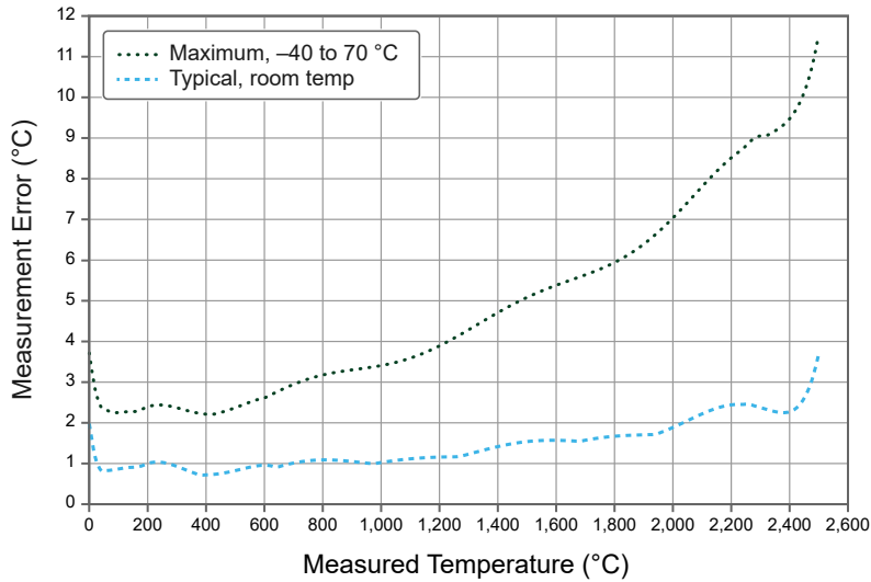
Figure 7. Thermocouple Types C and A Errors
