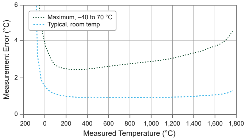
Figure 6. Thermocouple Types R and S Errors
